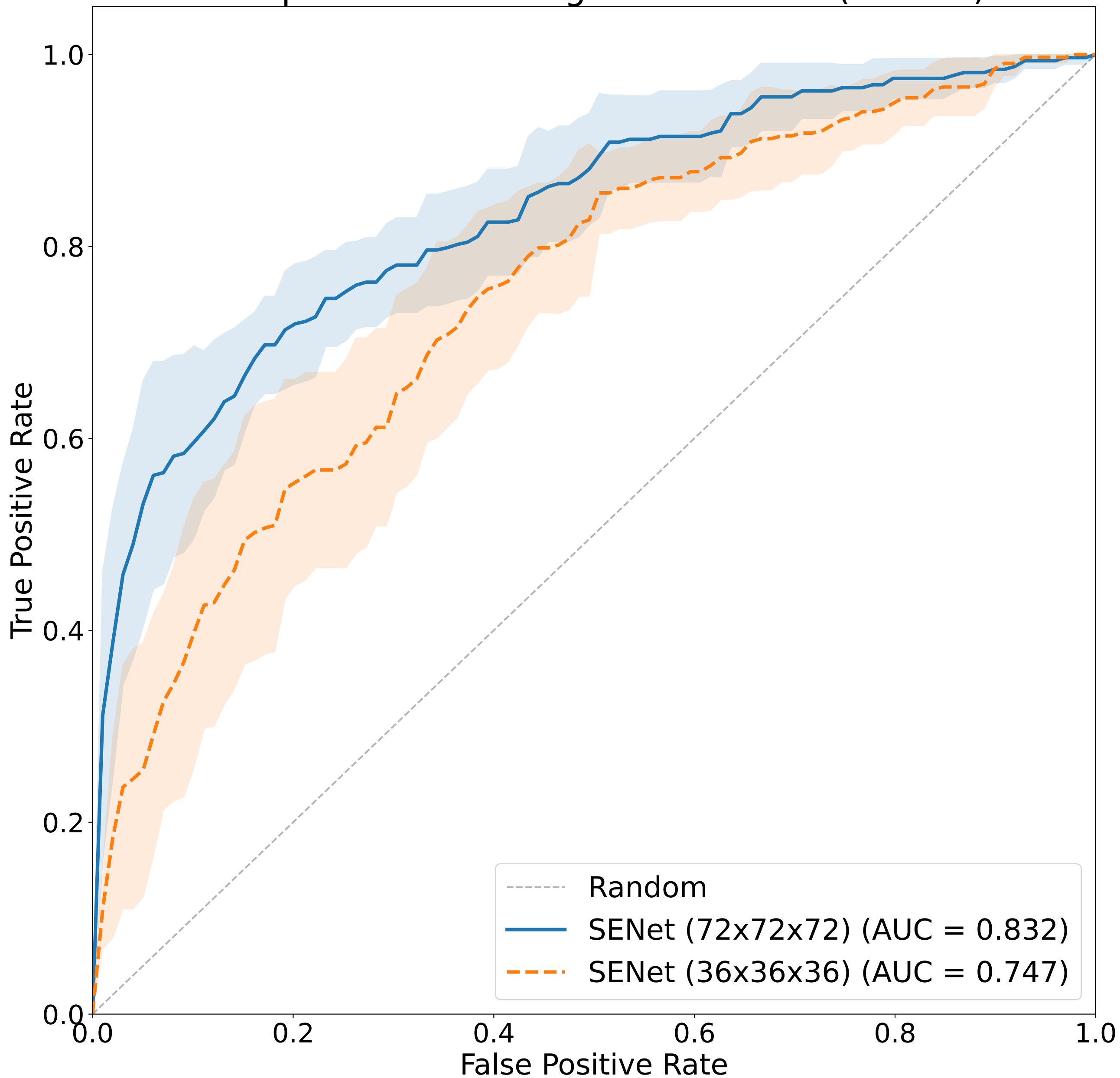
Comparison of Average ROC Curves (5 Folds)
